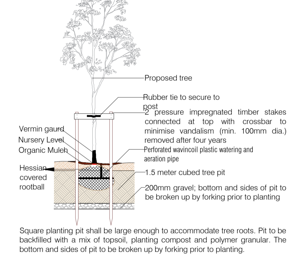
Detail 2: Standard Rootball Tree Planting Specification Not to Scale
