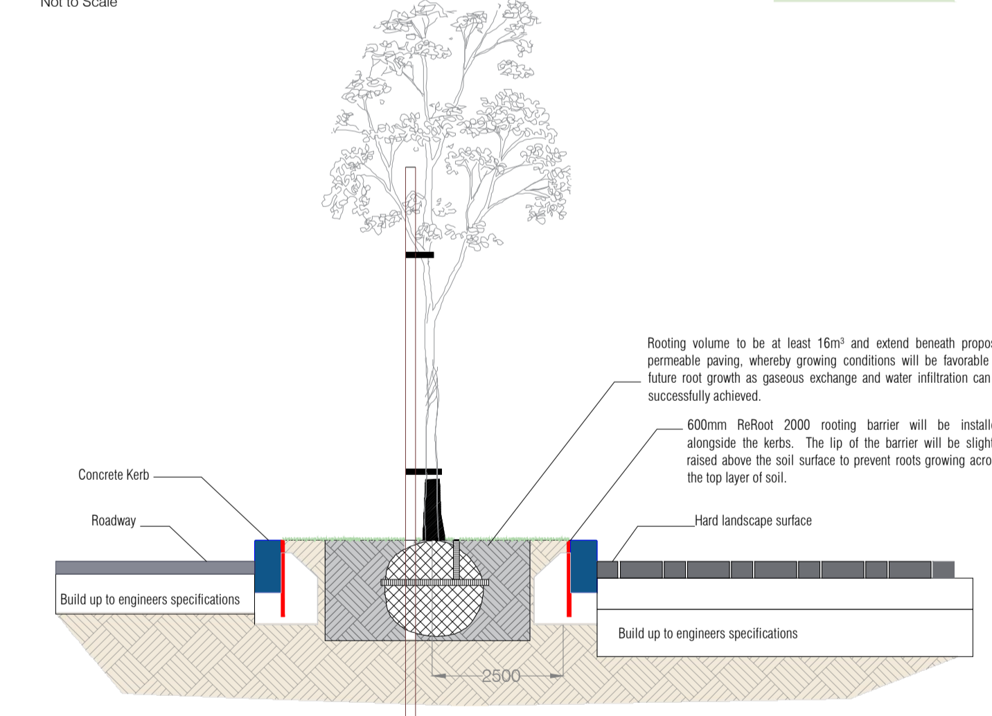
Single stake 12-14cm with root barrier Not to Scale
