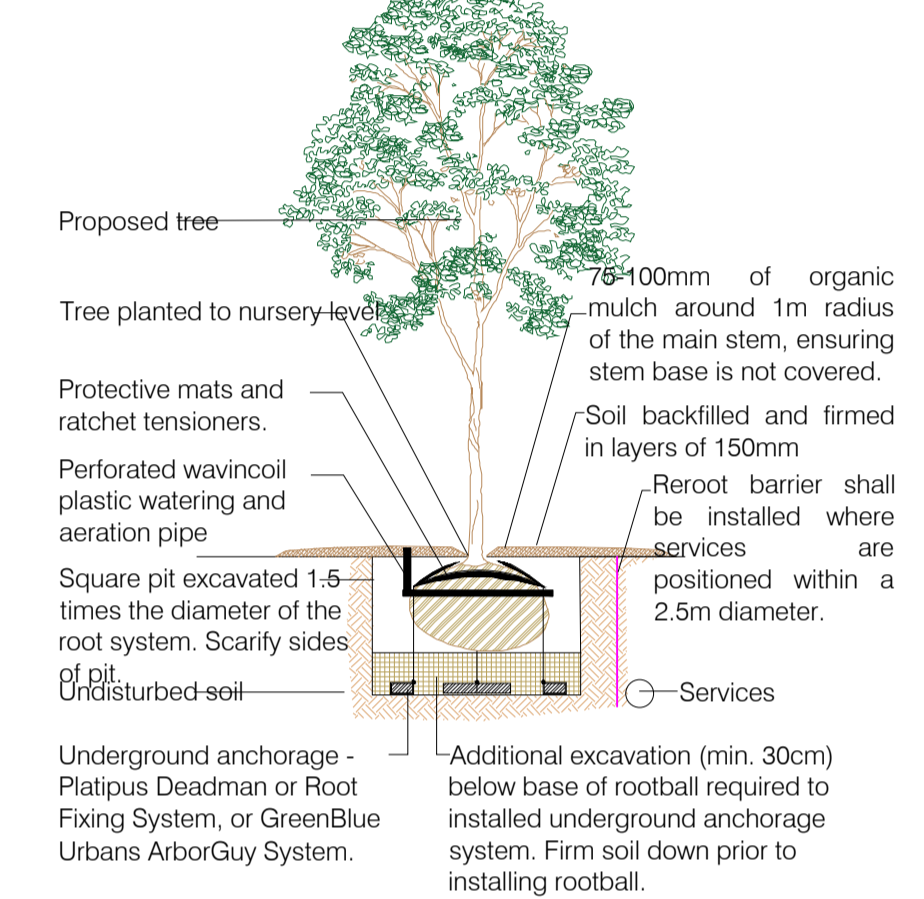
Detail 1: Tree Planting Underground Guying Not to Scale
